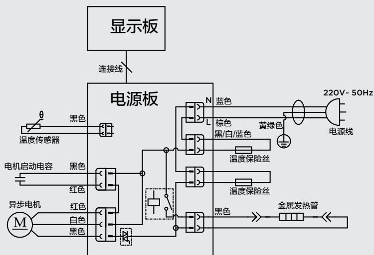
THS15BB-PW/AHS20AB-PG/THS20BB-PASY/AHS20AB-PT/ AHS20AB-PR电路图
