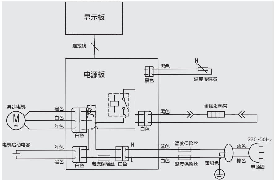
AHS15AC-PGS/AHS15AC-PAS/AHS15AC-PRSY/ AHS20AC-PASY电路图
